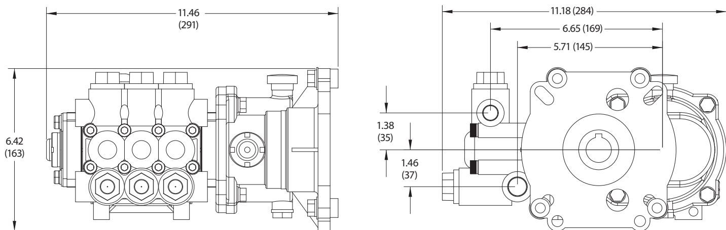
Model 5CP5135CSSG1 (with gearbox)
