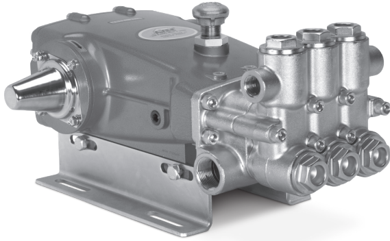
Model 2510.44101 Shown (Rails and shaft protector sold separately)
