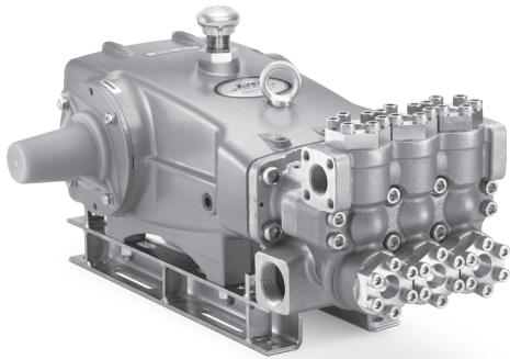
Model 3501.44101 Shown (Shaft protector included, mounting rails sold separately)
