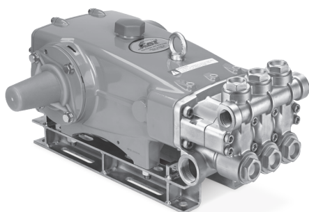
Model 3535 Shown (Shaft protector included, mounting rails sold separately)
