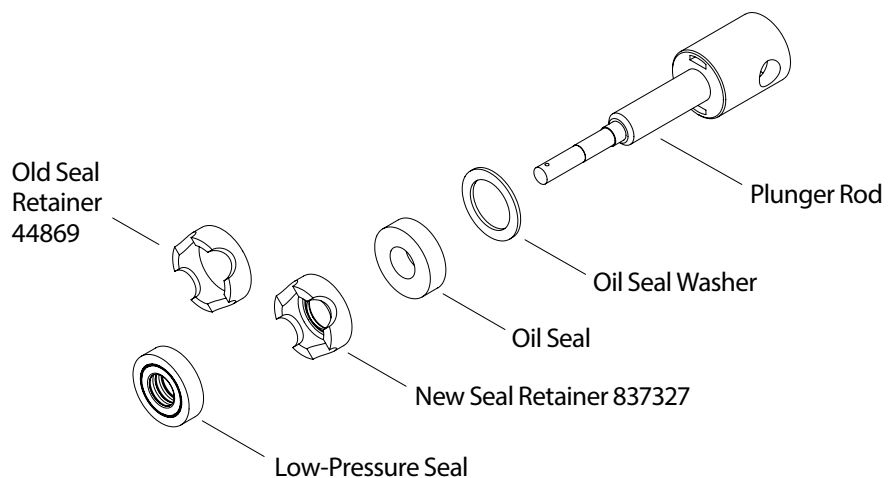
New Seal Retainer 837327
